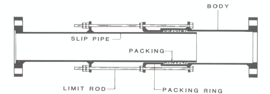
JCM 801 Single End Expansion Joint
